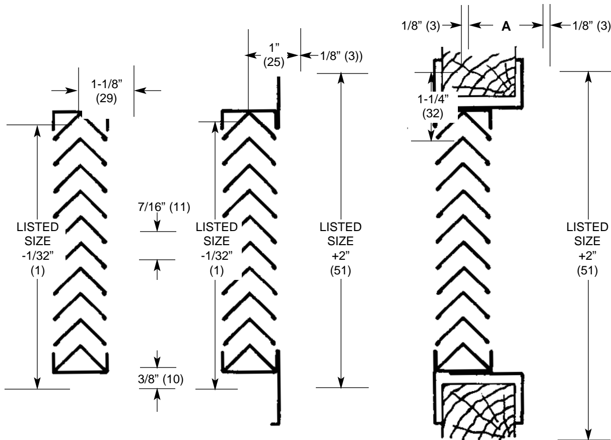
MODEL RGCAH with CHANNEL FRAME
