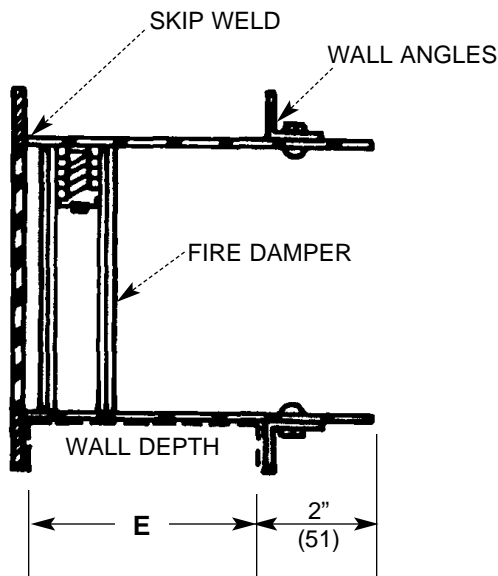
MODEL RSPA 03
