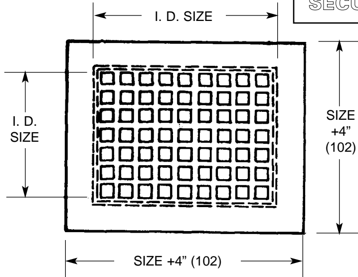
MODEL RSPA 03
